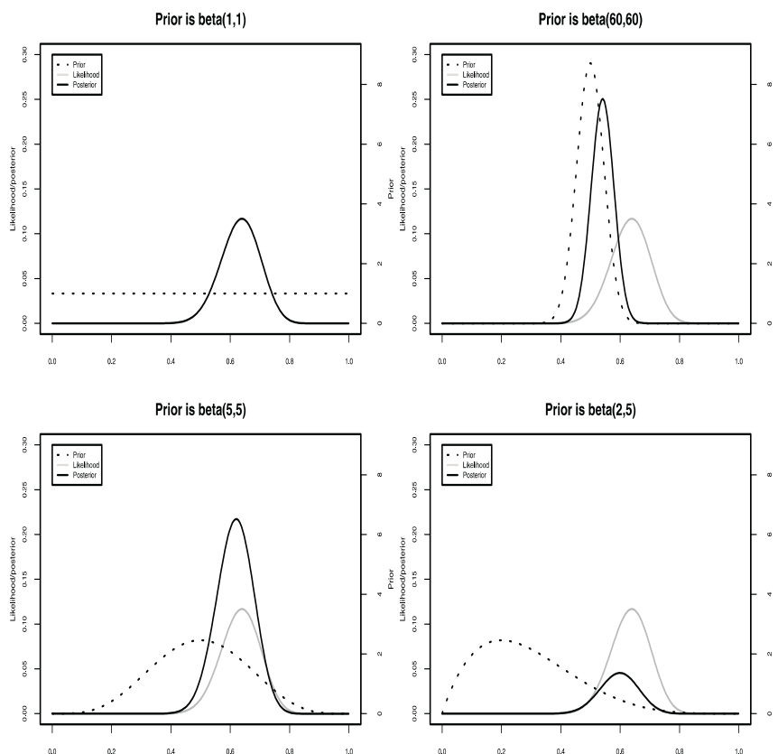
Figure 18. Posterior distributions for a set of four different prior distributions.
